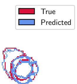
segmentations
